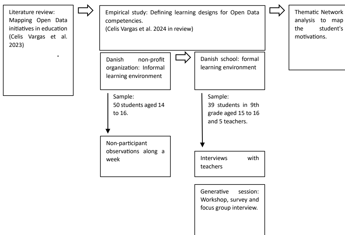
Figure 4: Methodological flow
